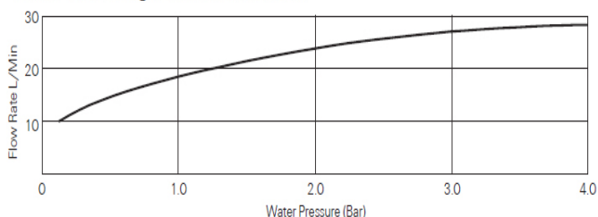
Talflo Discharge Characteristics
